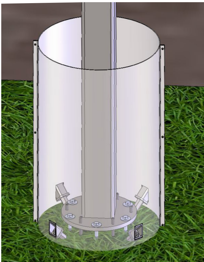
Fig. 24: Impact protection for the supports of the system in Heggelbach to protect against possible damage from farming machinery.
